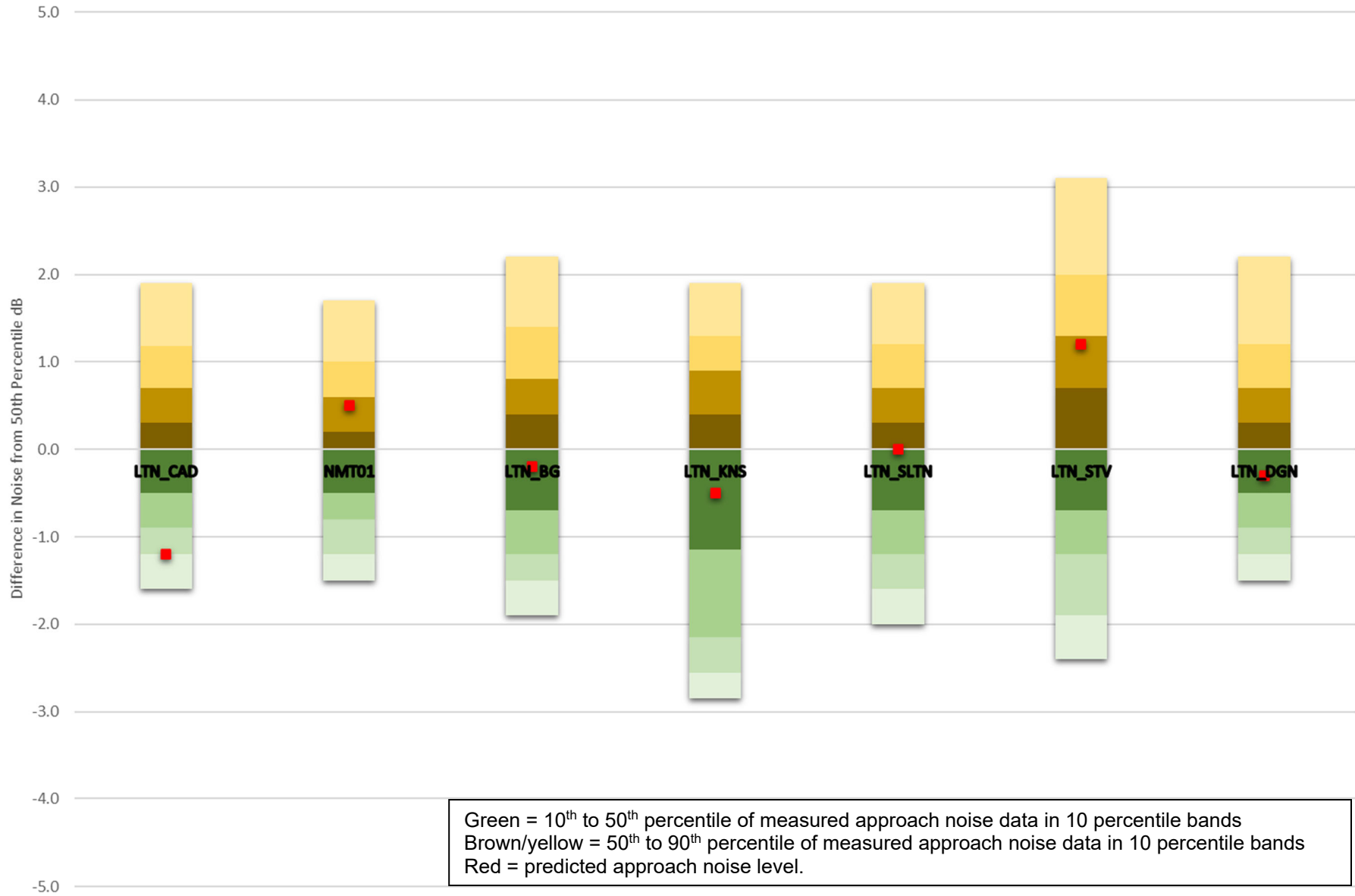
Inset 6.14: B737-800 L ASmax Approach Noise Testing
