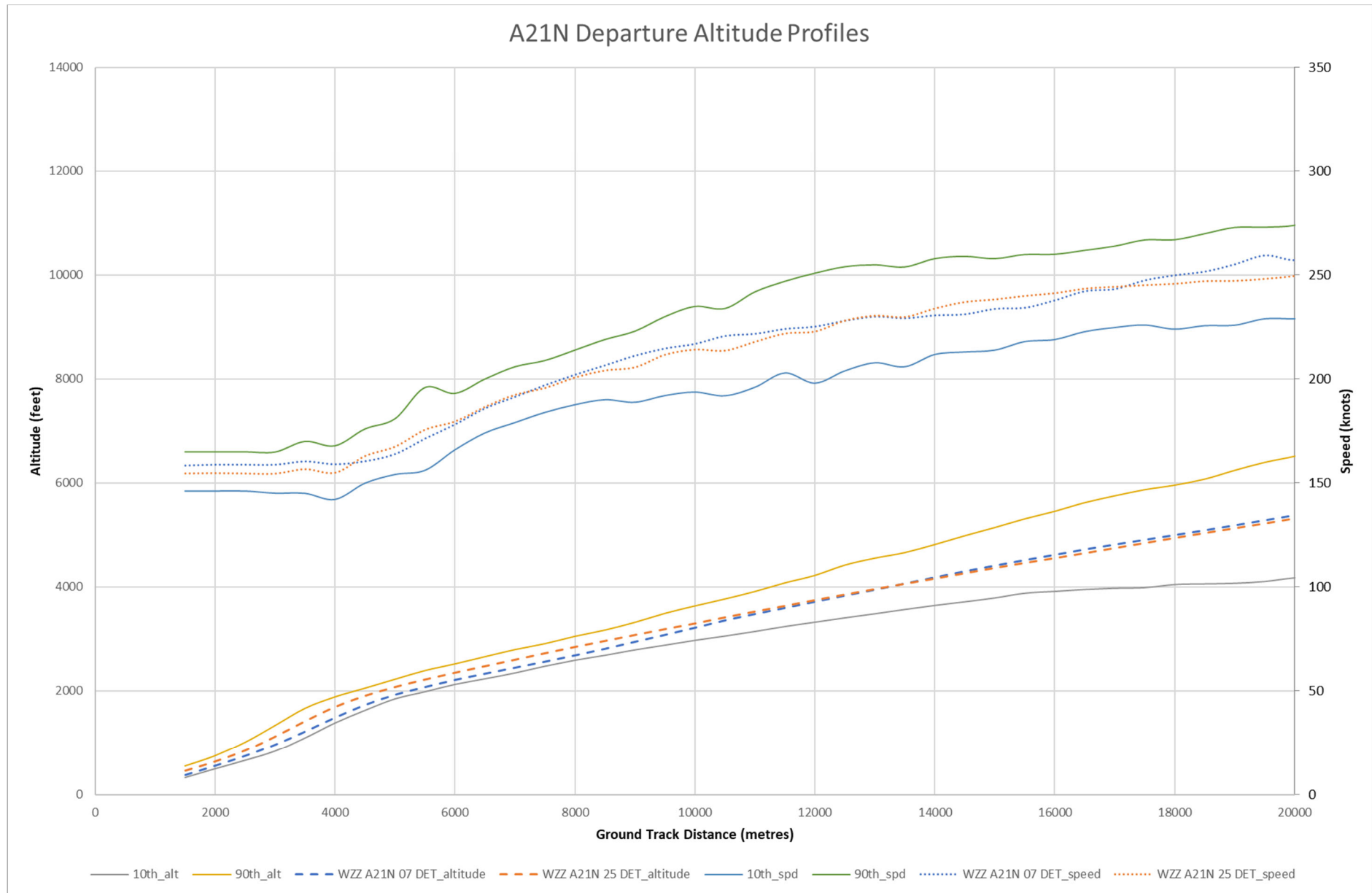
Inset 6.19: A321Neo Departure Profiles
