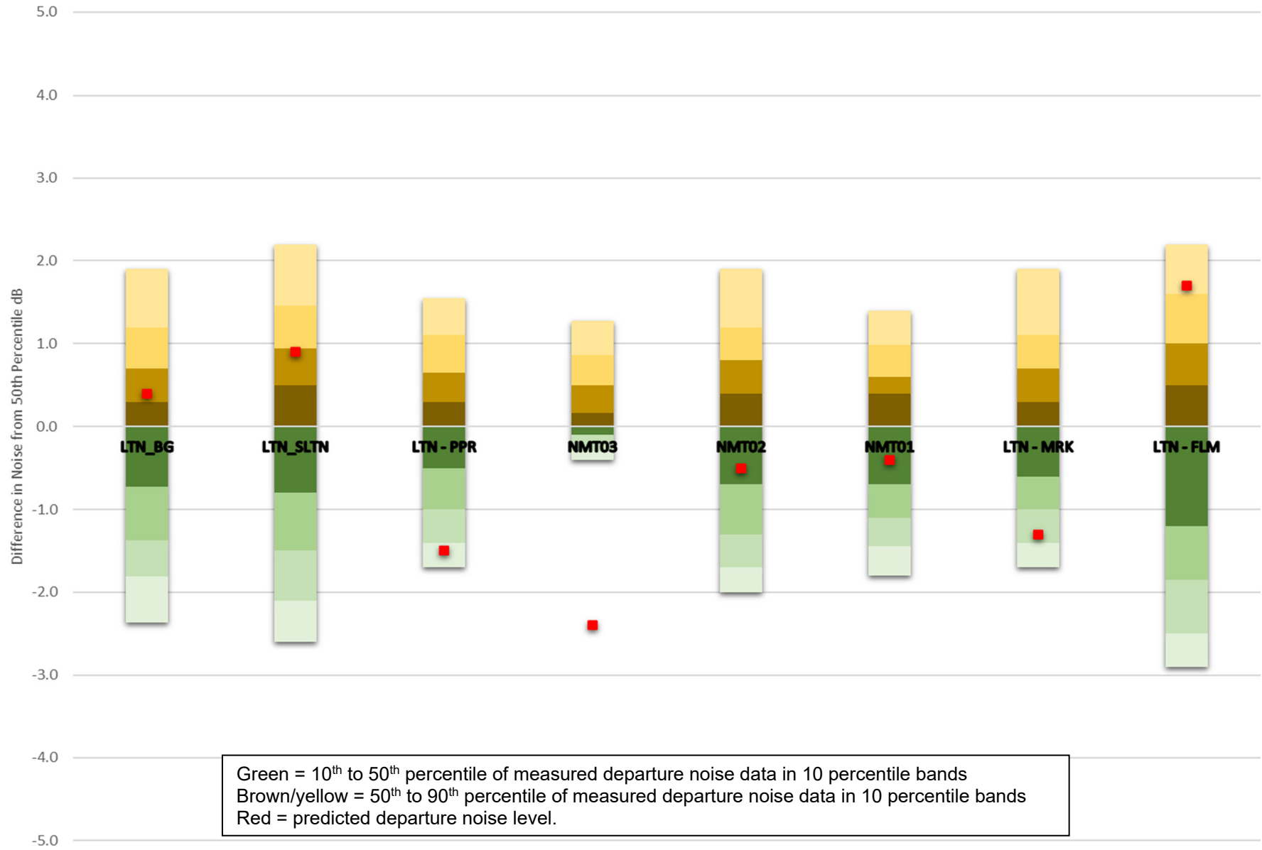
Inset 6.38: A320Neo L ASmax Departure Noise Testing
