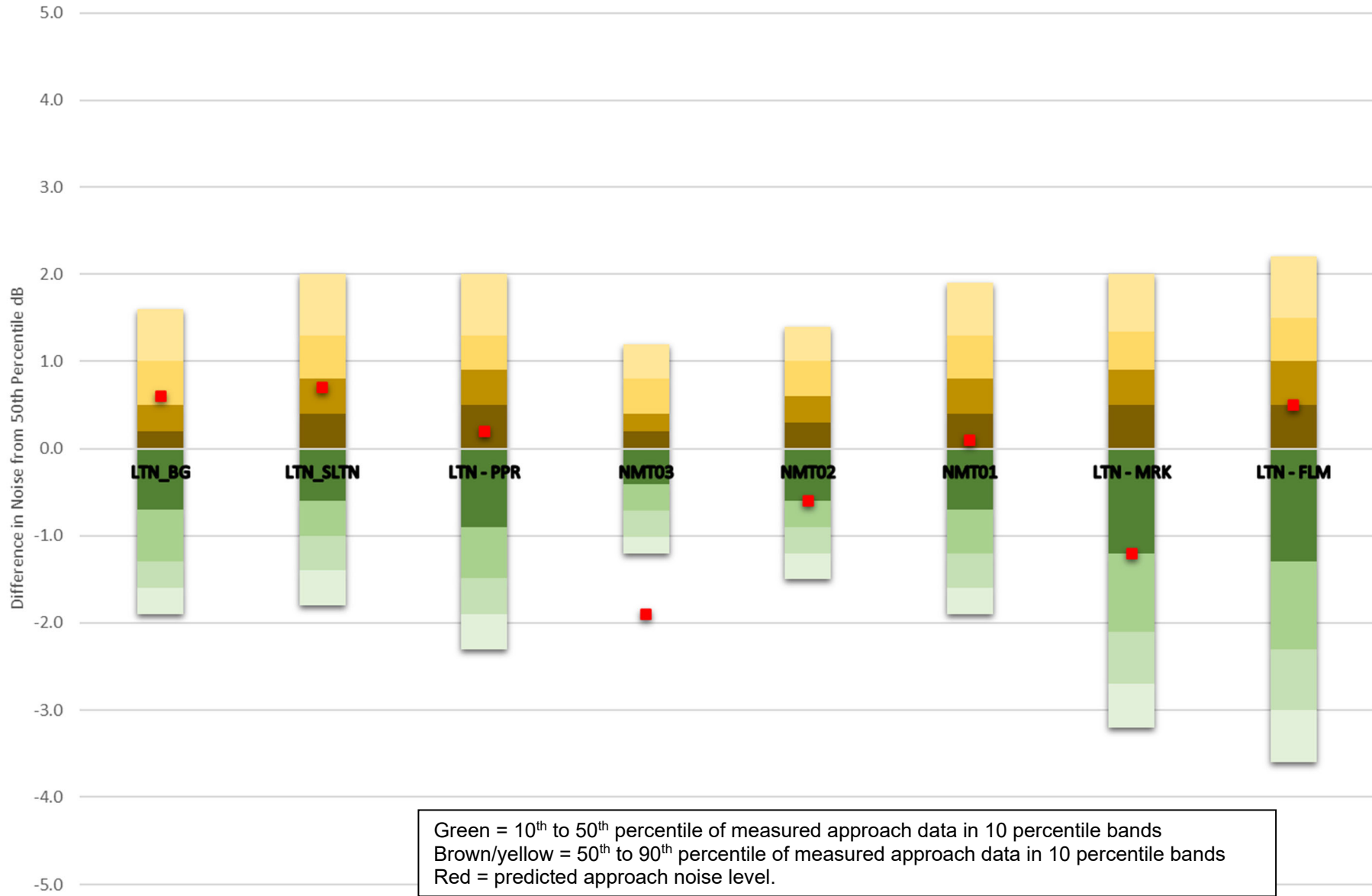
Inset 6.31: A320 SEL Departure Noise Testing
